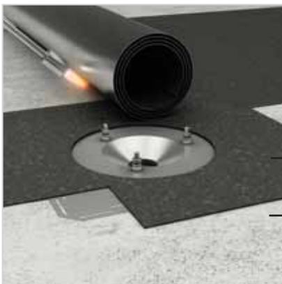
Bitumen Concrete/insulation
